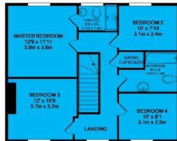
1ST FLOOR APPROX. FLOOR AREA 645 SQ.FT. (59.9 SQ.M.)
